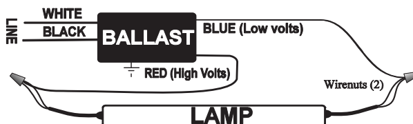
Figure 2- Typical Connections from Ballast for use with Preheat Lamps
