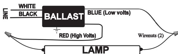
Figure 1- Typical Connections from Ballast for use with Instant Lamps
