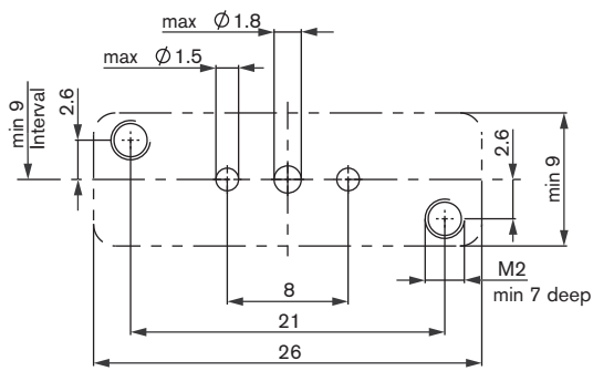
3/2 way connection
