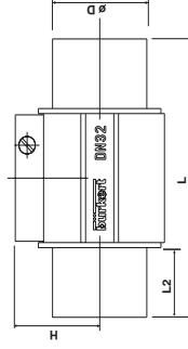
3.7: PVC/PP/PVDF connection; solvent/fusion spigot
