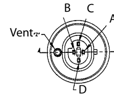
Top View: 4-Pin Packard Connector Type: Metri-Pack 150
