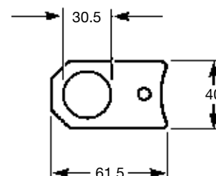
FK21 / FK28 fixing kit
