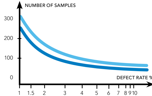
Fig. 3. The relation between defective product samples in percent and the total number of samples to be analysed for bacteria needed to find one or more defects in samples at 90 and 95% levels of probability.
