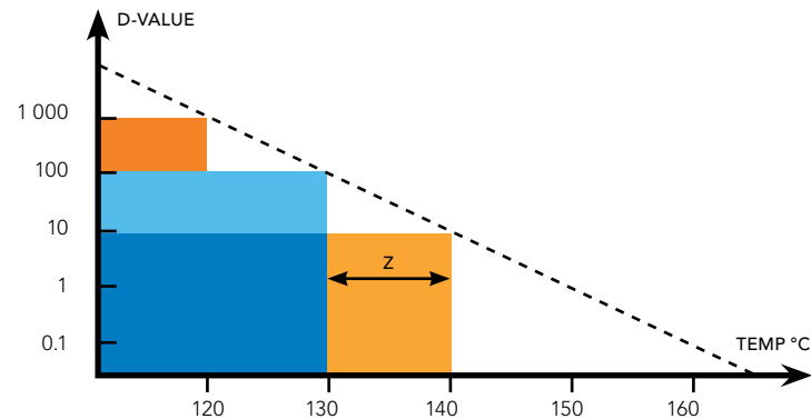
Fig. 2. The Z-value is the increase in temperature needed to achieve the same lethal action or the same effect in one-tenth of the time.
