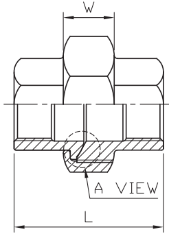
Conical union
