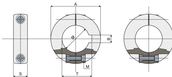
With Keyway
